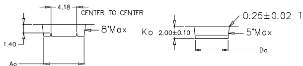
DETAIL 'A'
